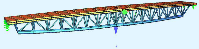
Structural model
