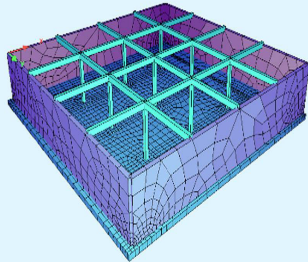
Structural model
