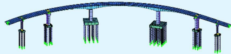
Structural model NRA unit 2
