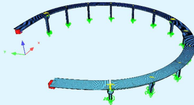
Structural model
