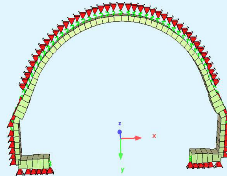
Structural model
