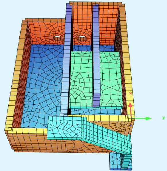
Structural model
