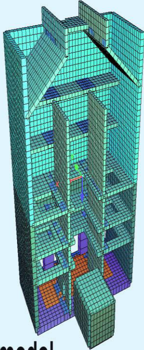
Structural model
