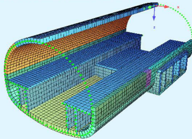
Structural model metro Athens
