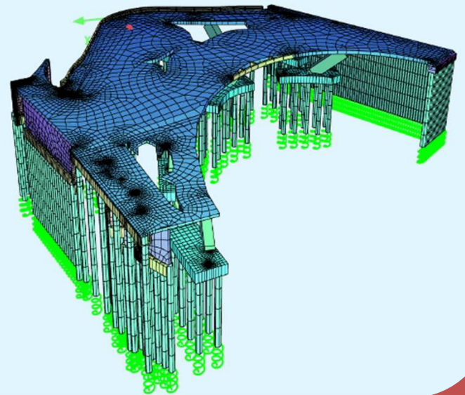
Structural model
