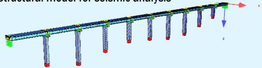
Structural model for seismic analysis
