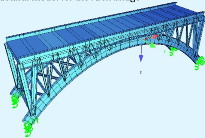
Structural model for the Arch bridge
